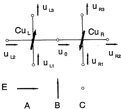
FIG. 2. Schematic representation of the cluster used in the calculations. Full dots represent Cu's and open dots O's. Thick arrows represent the spin, thin short arrows represent lattice displacements, and thin long arrows represent the direction of the electric field. We have represented u_0 in A configuration. In general its direction is equal to the direction of the electric field.
