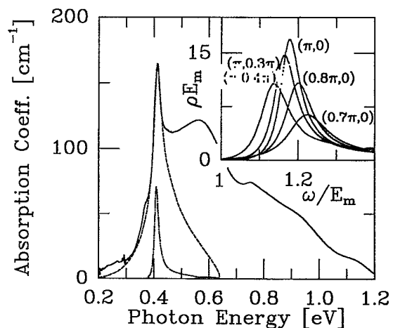
FIG. 1. Experimental data from Ref. [3] (solid line) and theoretical line shape for two-magnon absorption (dashed line) in \text{La}_2\text{CuO}_4 . The dash-dotted line is the contribution to the line shape from the bimagnon at p = (\pi, 0) . The inset shows a blowup of \rho = -\text{Im}(G_{xx}) at the energy of the bimagnon for different values of the total momentum.
