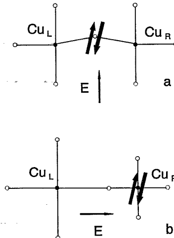
FIG. 3. Typical processes contributing to the isotropic (a) and anisotropic (b) effective charges. The meaning of the symbols is the same as in Fig. 2.
